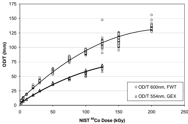
Figure 8. Sensitivity of OD/T to absorbed dose – full range.
