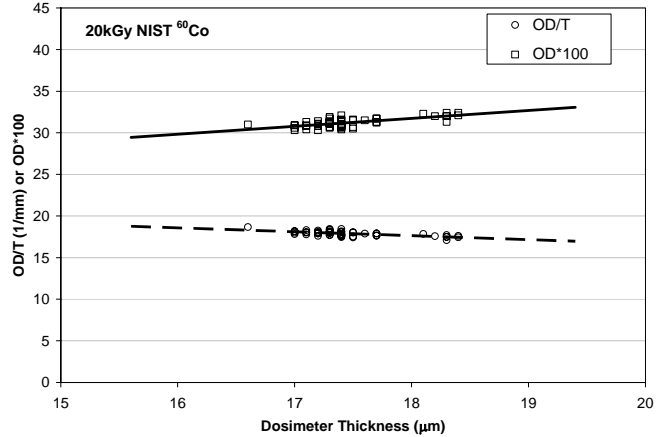
Figures 4 and 5. Dependence of optical density change (OD) and normalized metric (OD/T) on thickness for 20kGy exposed FWT (left) and GEX (right) dosimeters.
