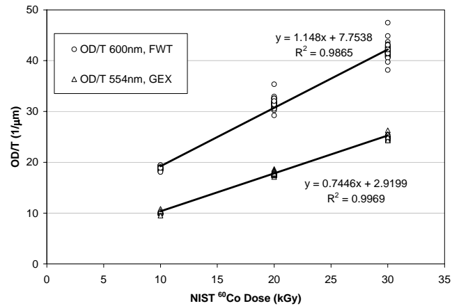
Figure 9. Sensitivity at lower dose regime.
