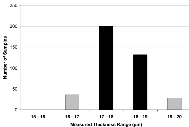
Figures 2 and 3. Distribution of thicknesses of FWT dosimeters (left) and GEX dosimeters (right).
