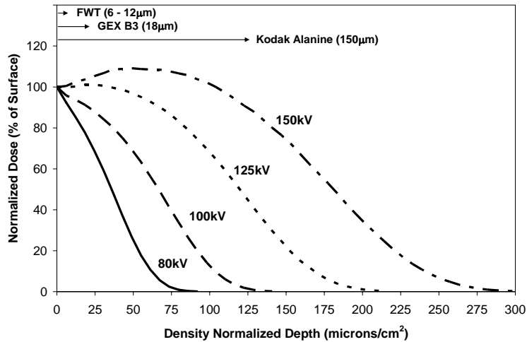
Figure 1: calculated dose-depth curves for LVEB irradiating unit density material.
