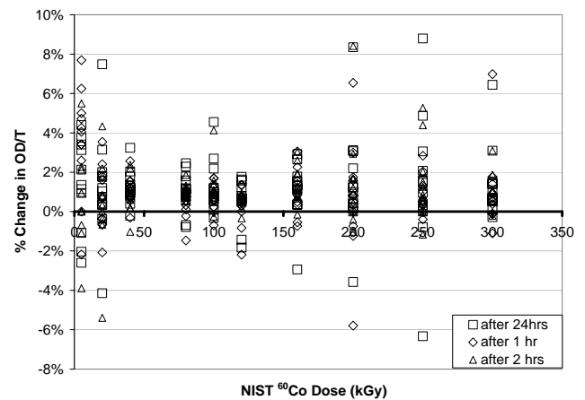
Figure 6. Impact of stabilization protocol on measured OD/T. Figure 7. Impact of post-stabilization measurement time.
